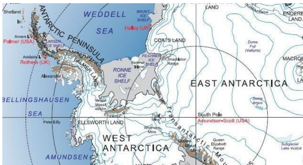
Figure 1: Antarctica Map
